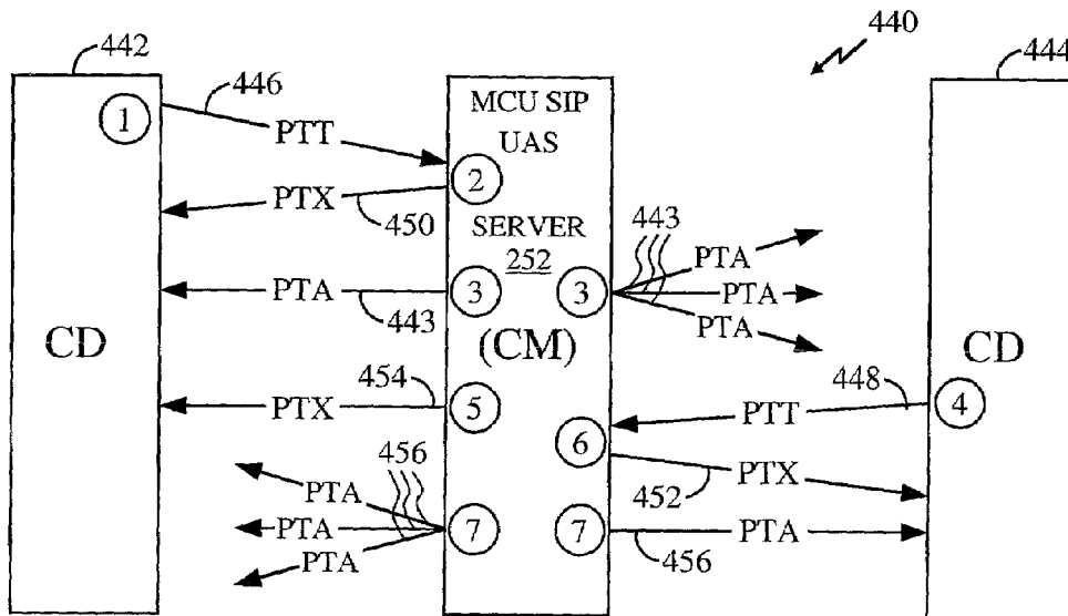
MEDIA SIGNALING MESSAGE SEQUENCE (PRIORITY ARBITRATION)
